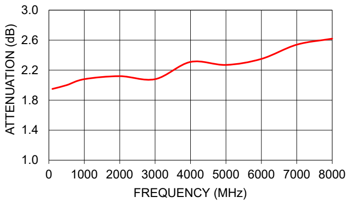
GAT-2+ ATTENUATION
