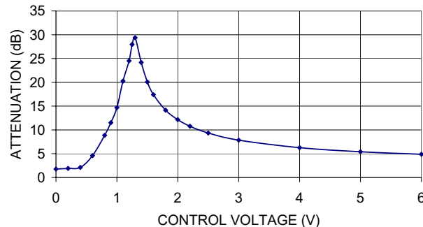
HVA-73+ TYPICAL ATTENUATION at 6260 MHz
