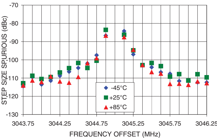
0.5 STEP SIZE & STEP SIZE SPURIOUS Vs FREQ. OFFSET @ Fcar = 3045MHz
