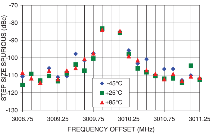
0.5 STEP SIZE & STEP SIZE SPURIOUS Vs FREQ. OFFSET @ Fcar = 3010MHz
