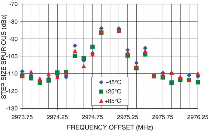
0.5 STEP SIZE & STEP SIZE SPURIOUS Vs FREQ. OFFSET @ Fcar = 2975MHz
