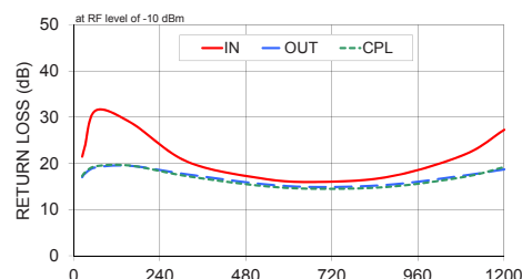
LRDC-10-2W-75+ RETURN LOSS
