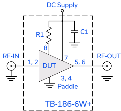
Fig 1. Block Diagram of Test Circuit used for characterization. (DUT soldered on Mini-Circuits Characterization test board TB-186-6W+) Gain, Return Loss, Output Power at 1 dB Compression (P1dB), Output IP3 (OIP3) and Noise Figure measured using Agilent's N5242A PNA-X microwave network analyzer.
