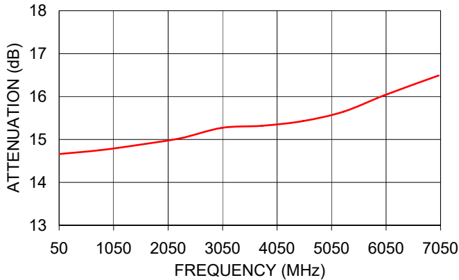
PAT-15+ ATTENUATION
