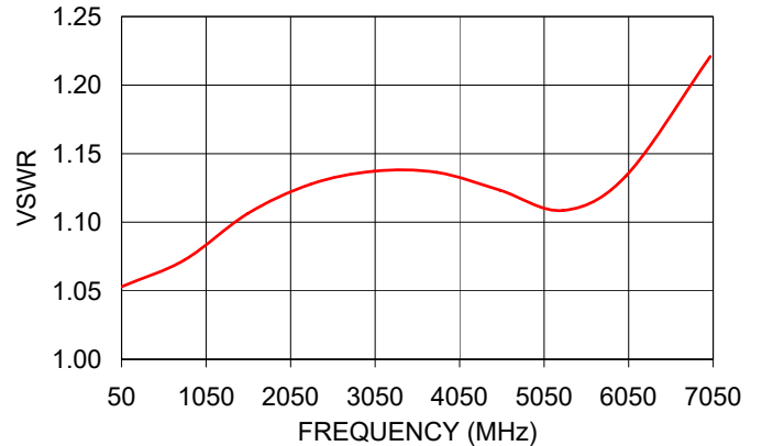
PAT-15+ VSWR
