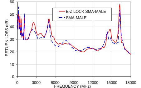
QBL1.5SMQ-SM+ RETURN LOSS
