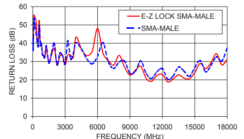
QBL1MSMQ-SM+ RETURN LOSS
