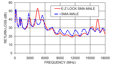
QBL3SMQ-SM+ RETURN LOSS
