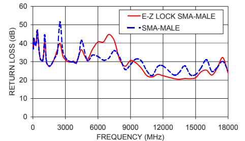
QBL4SMQ-SM+ RETURN LOSS
