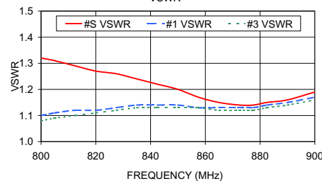
ZB6PD1-900 VSWR
