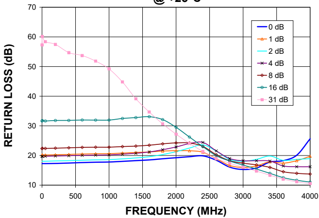
RETURN LOSS IN (Major Atten. Steps) @ +25°C
