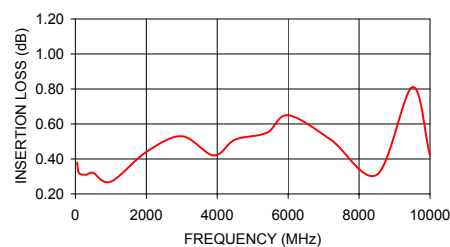
INSERTION LOSS
