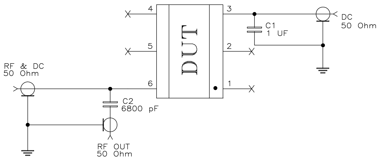
Schematic Diagram
