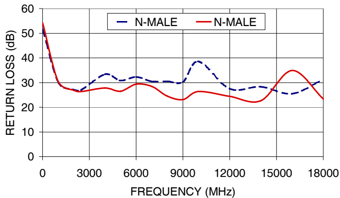
CBL-1.5M-NMNM+ RETURN LOSS
