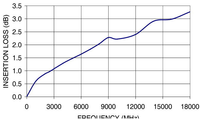
CBL-1.5M-NMNM+ INSERTION LOSS
