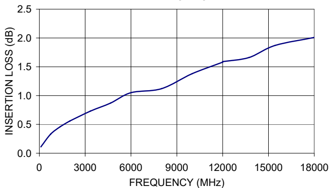
CBL3NMQ-NM+ INSERTION LOSS
