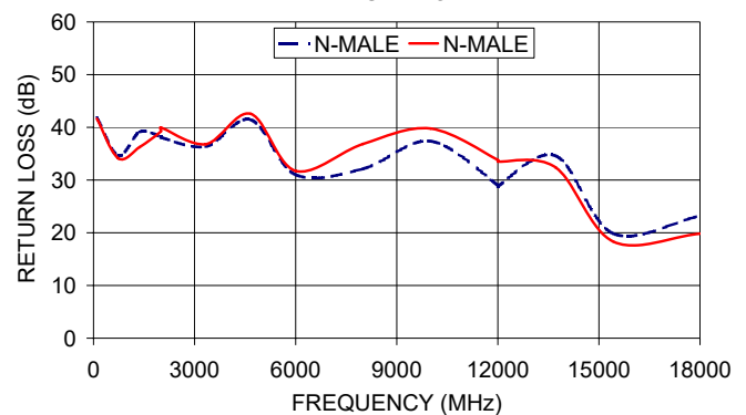
CBL3NMQ-NM+ RETURN LOSS
