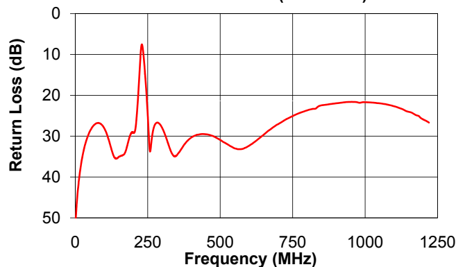
DPB204258-75+ COMMON PORT RETURN LOSS ( P_{in}=0\text{dBm} )
