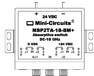
Marking Drawing
