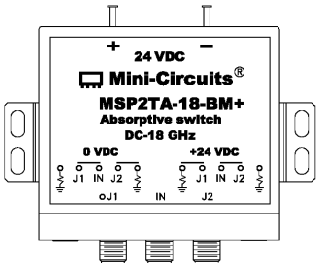
Marking Drawing
