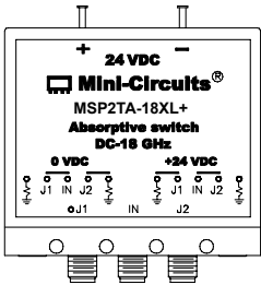
Marking Drawing
