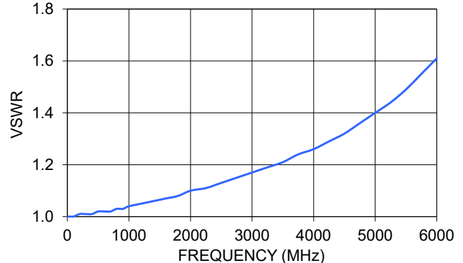
VAT-15W2+ VSWR
