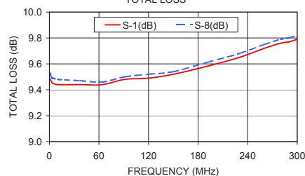
ZFSC-84-75+ TOTAL LOSS
