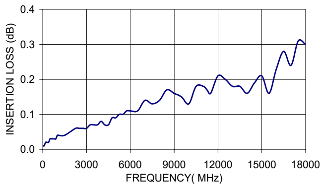
141-3SM+ INSERTION LOSS
