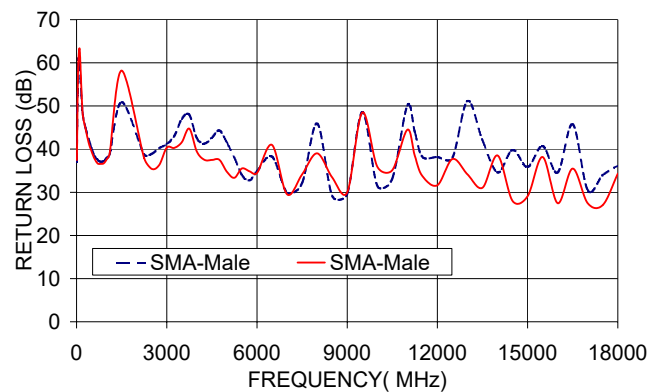
141-3SM+ RETURN LOSS
