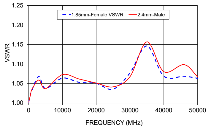
185F-24M+ VSWR
