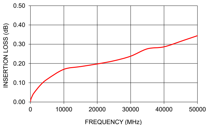
185F-24M+ INSERTION LOSS
