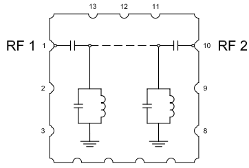
Figure 1. CBP2-1090C+ Functional Diagram
