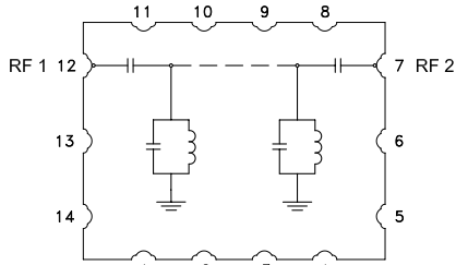
Figure 1. CBP2-1300BV+ Functional Diagram
