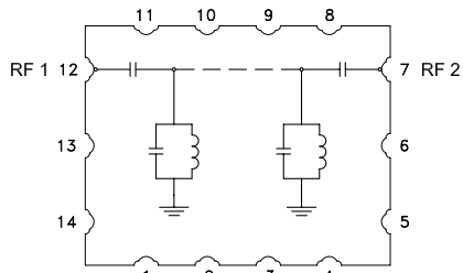
Figure 1. CBP2-1300BV+ Functional Diagram
