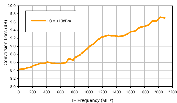
Conversion Loss vs. IF @ RF=2100.1MHz
