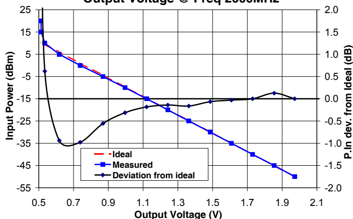
Power Input Deviation from Ideal Vs Output Voltage @ Freq 2000MHz
