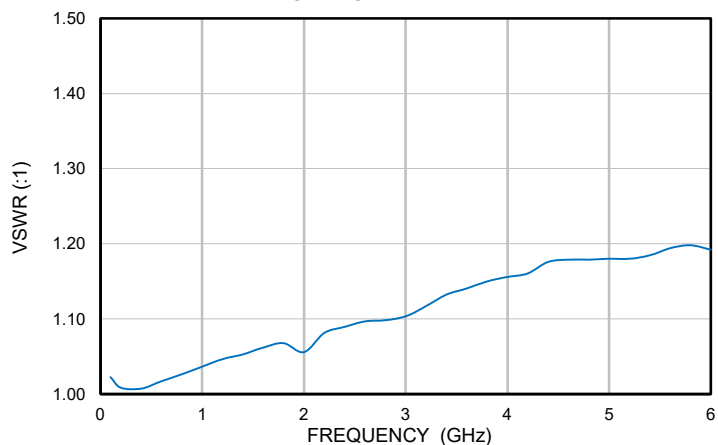
Right Angle MCX VSWR (+25°C)
