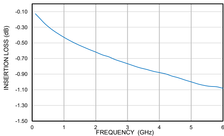
INSERTION LOSS (+25°C)
