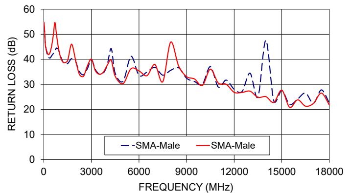
086-4SM+ RETURN LOSS
