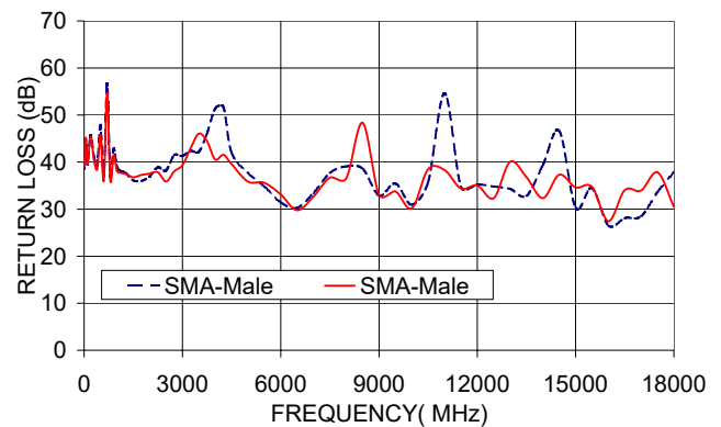
141-18SM+ RETURN LOSS
