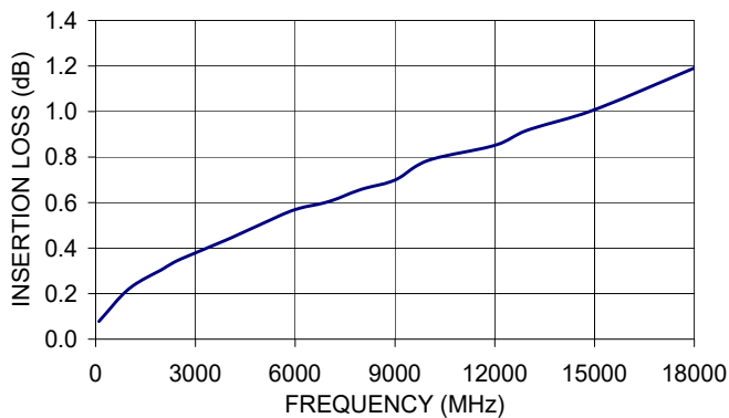
141-20SM+ INSERTION LOSS
