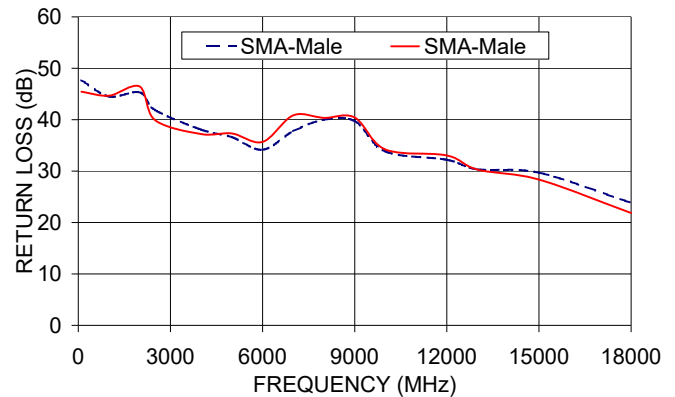
141-20SM+ RETURN LOSS
