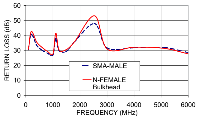
141-24SMNB+ RETURN LOSS
