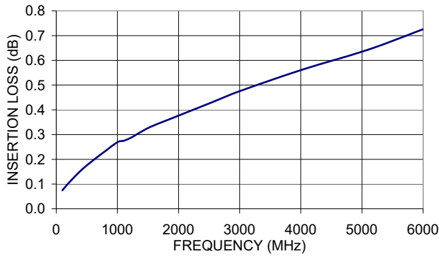
141-24SMNB+ INSERTION LOSS
