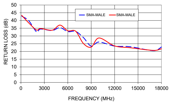
141-32SM+ RETURN LOSS
