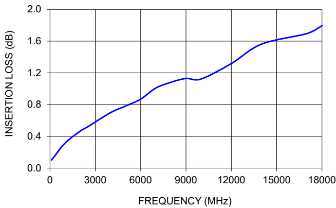
141-32SM+ INSERTION LOSS
