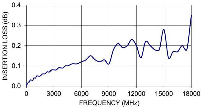
141-4SM+ INSERTION LOSS
