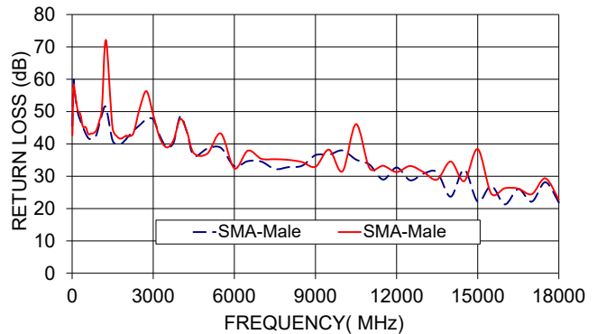
141-4SM+ RETURN LOSS
