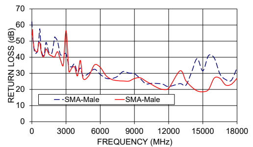
141-7SM+ RETURN LOSS
