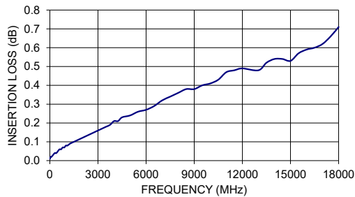
141-7SM+ INSERTION LOSS
