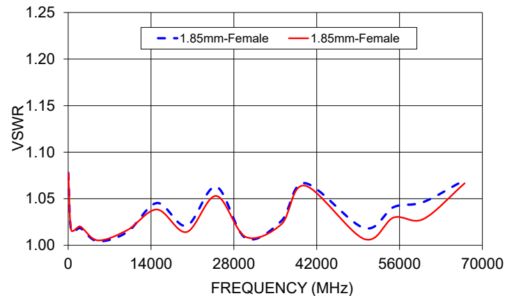
185F-185F+ VSWR
