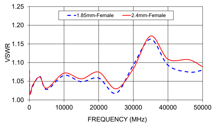
185F-24F+ VSWR
