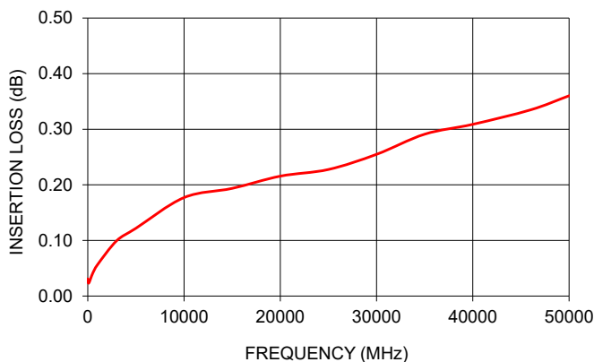
185F-24F+ INSERTION LOSS
