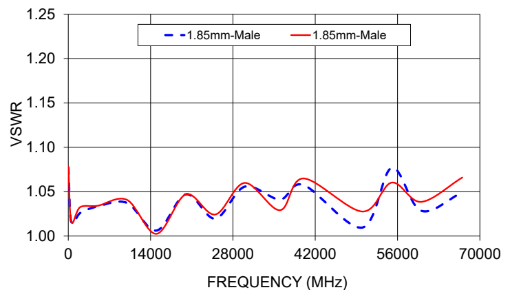
185M-185M+ VSWR
