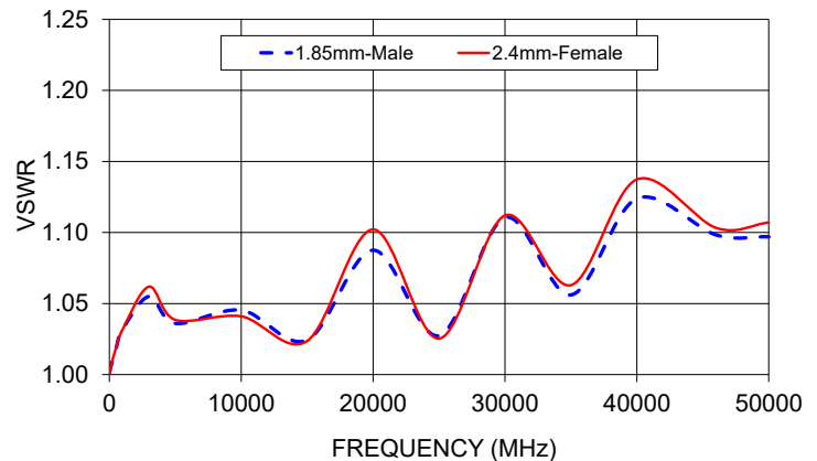
185M-24F+ VSWR
