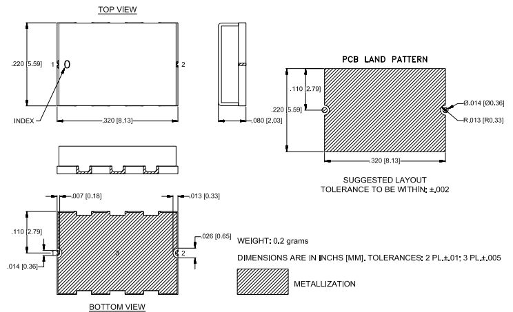
CASE STYLE DRAWING
