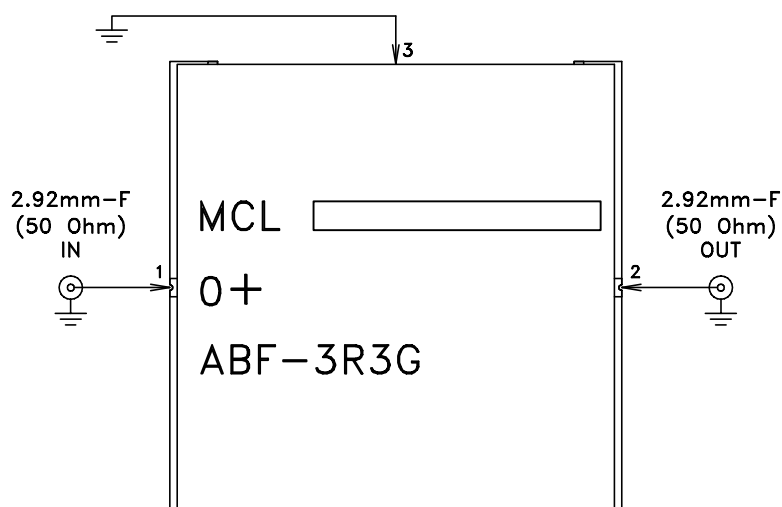
Schematic diagram
