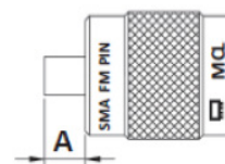
Fig 2. Gaging a Female SMA Connector
