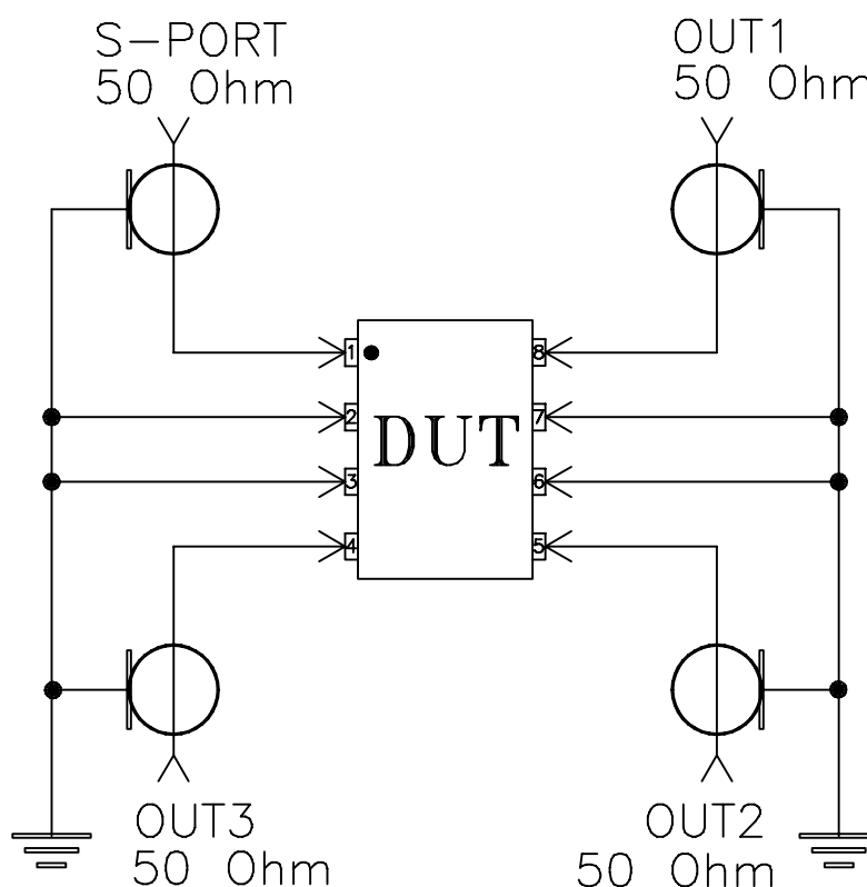
Schematic Diagram
