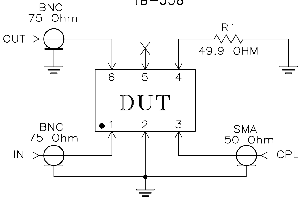
Schematic Diagram
