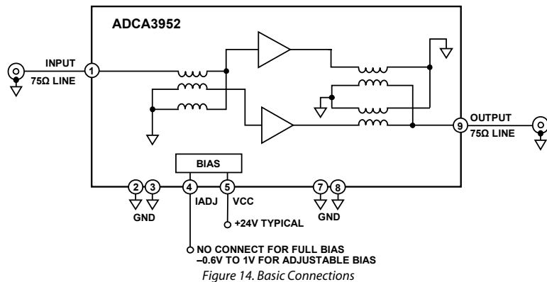
Figure 14. Basic Connections
