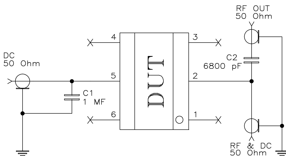
Schematic Diagram
