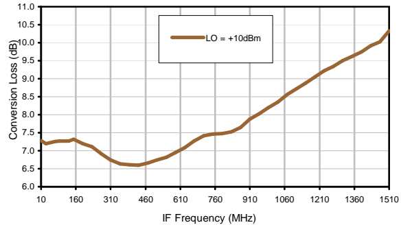
Conversion Loss vs. IF @ RF=1520.1MHz
