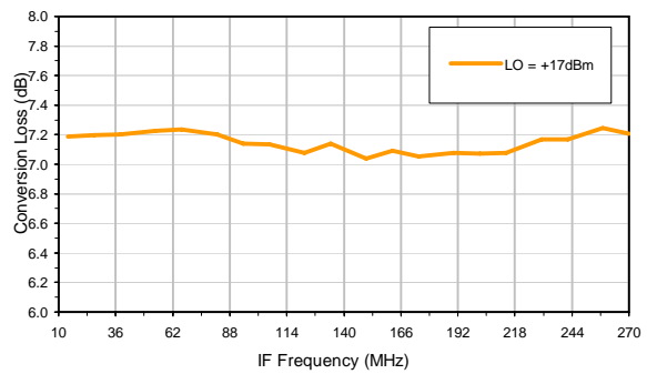
Conversion Loss vs. IF @ RF=367.1 MHz
