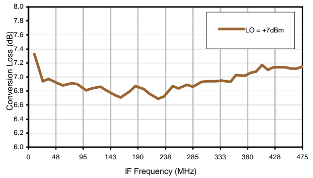
Conversion Loss vs. IF @ RF=485.1MHz
