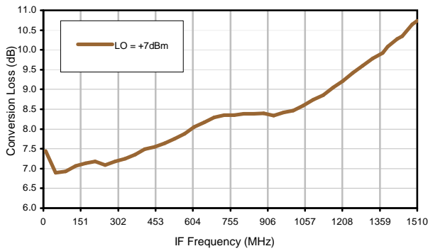
Conversion Loss vs. IF @ RF=70.1MHz
