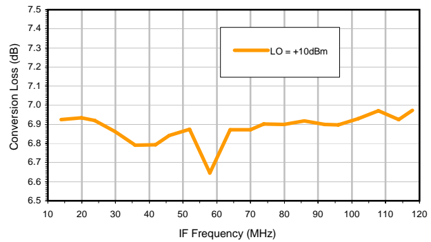
Conversion Loss vs. IF @ RF=246 MHz
